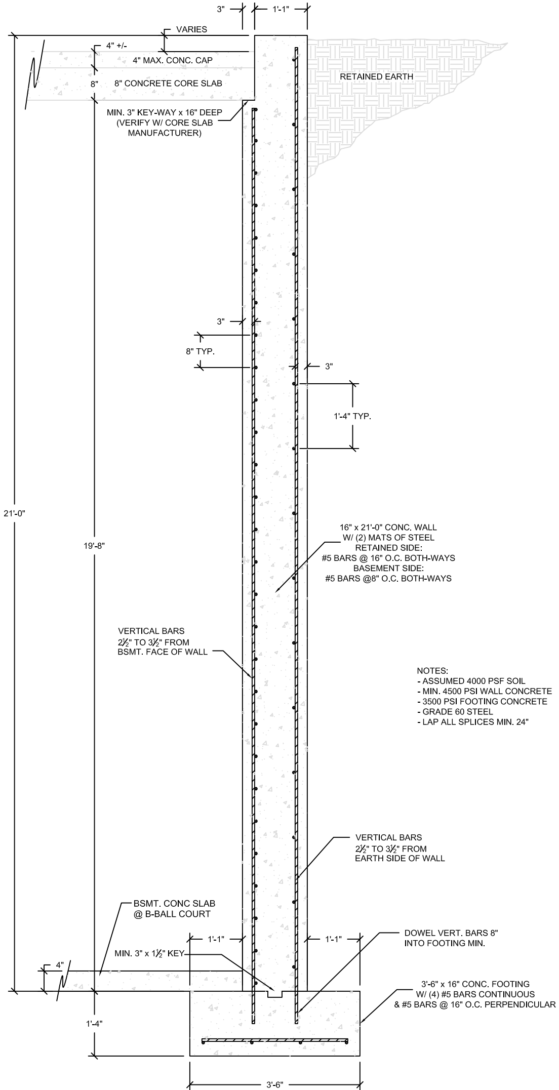
16" X 21'-0" CONC. FOUNDATION WALL DETAIL NOT TO SCALE
